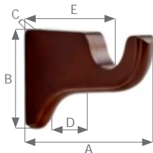
2" WALL BRACKET
