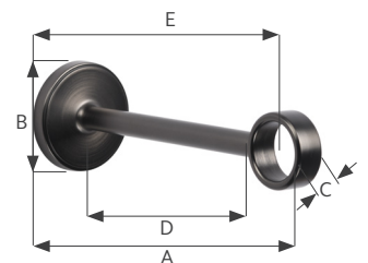
6" Return 1" O Bracket
