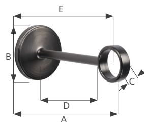
6" Return 1 \frac{3}{8} " O Bracket
