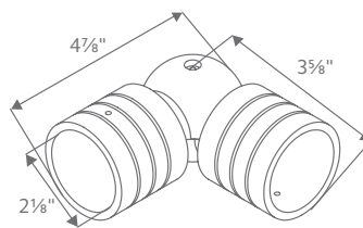
2" SWIVEL SOCKET
