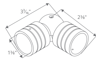
1 3/8" SWIVEL SOCKET
