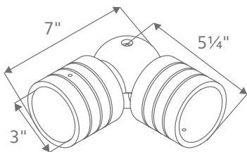
3" SWIVEL SOCKET
